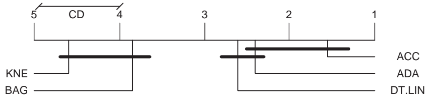
Fig. 8. Graphical representation of post-hoc Nemenyi test results of compared methods with ranks given in Table 17
